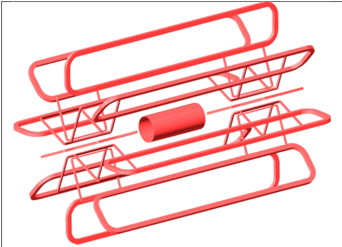
Figure 7 : The magnets used by ATLAS
