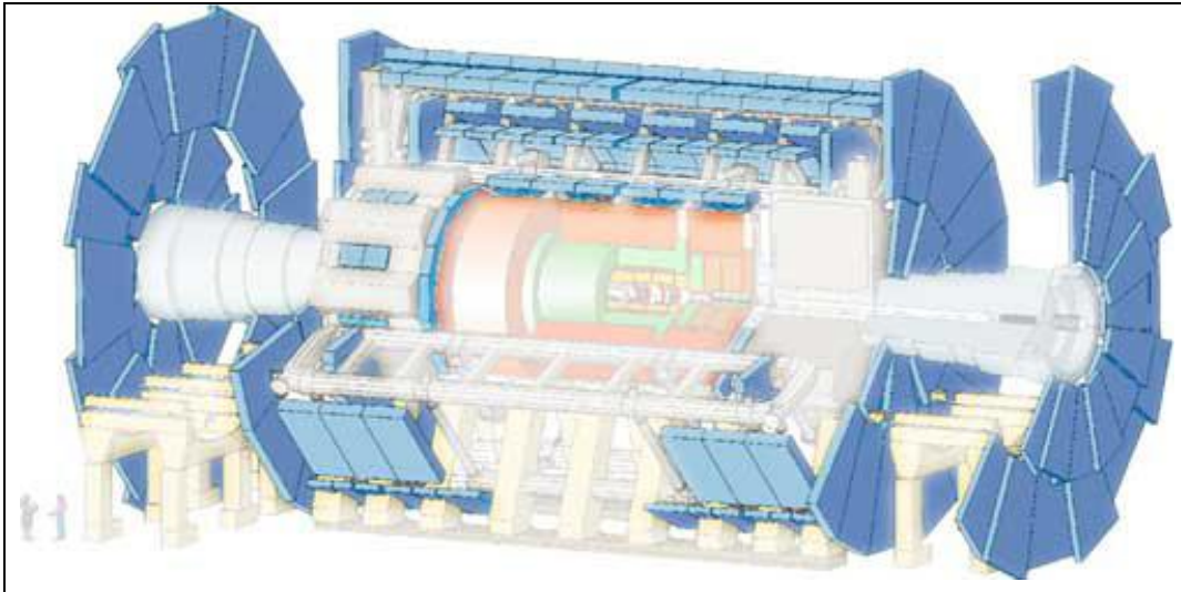
Figure 5 : Muon Chambers
