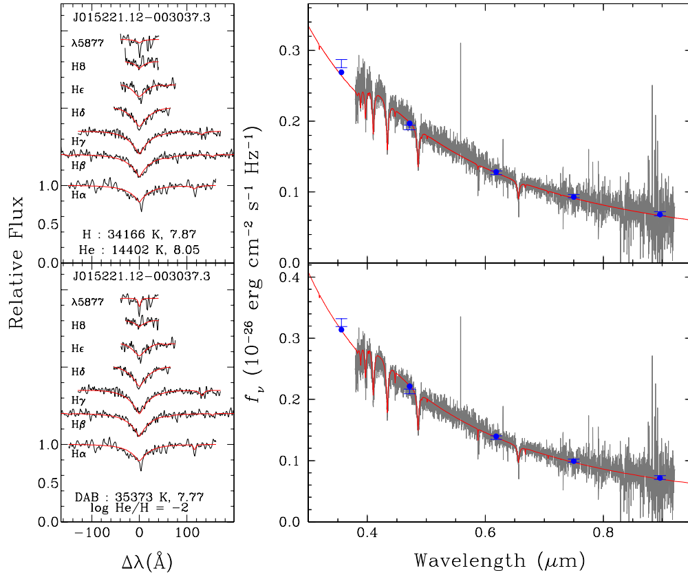
Figure 13. Top: our DA+DB solution for J015221.12-003037.3. The left panel shows our best spectroscopic fit reproduced from Figure 10, while the right panel shows the superposition of the observed and predicted photometry (only the scaling factor is adjusted here) using the same presentation format as previous figures. Bottom: our DAB homogeneous solution for the same object. The left panel shows our spectroscopic fit with an assumed helium abundance of \text{He}/\text{H} = 10^{-2} . Again, the right side represents a superposition of the observed and predicted photometry using the spectroscopic atmospheric parameters. (A color version of this figure is available in the online journal.)
