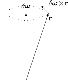
Figure 1.2: \delta\boldsymbol{\omega} \times \mathbf{r} is perpendicular to \delta\boldsymbol{\omega} and \mathbf{r} , and represents an infinitesimal rotation of \mathbf{r} about the \delta\boldsymbol{\omega} axis.
