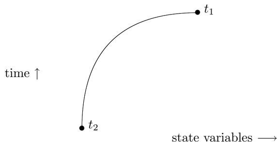
Figure 1.1: A possible path from initial state to final state.
